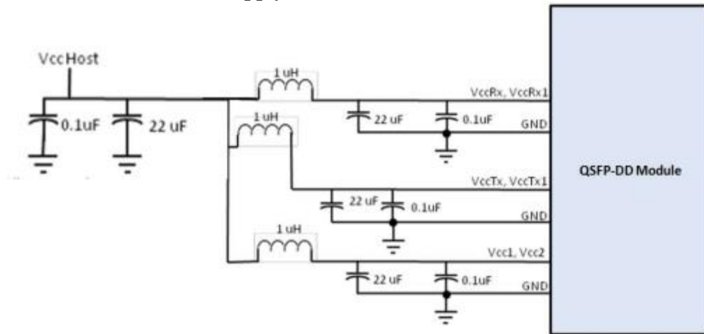
Figure 4. Recommended Power Supply Filter
