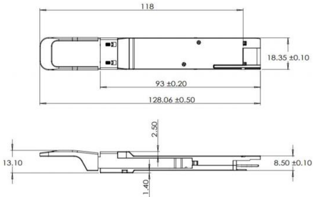
Figure 6. Mechanical Outline
