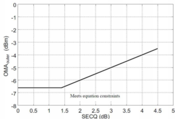
Figure 5. RX sensitivity
