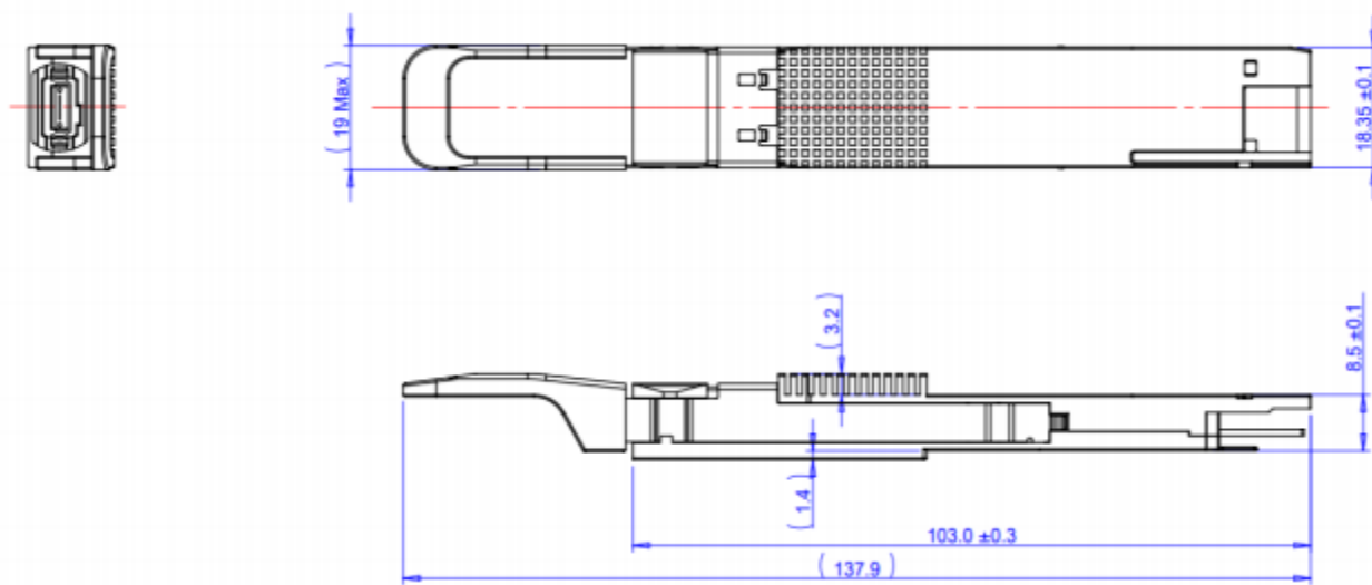
Figure 5. Mechanical Outline
