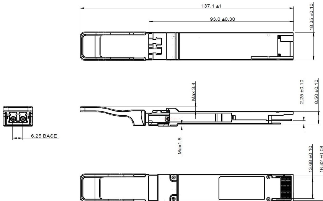
Figure 5. Mechanical Outline
