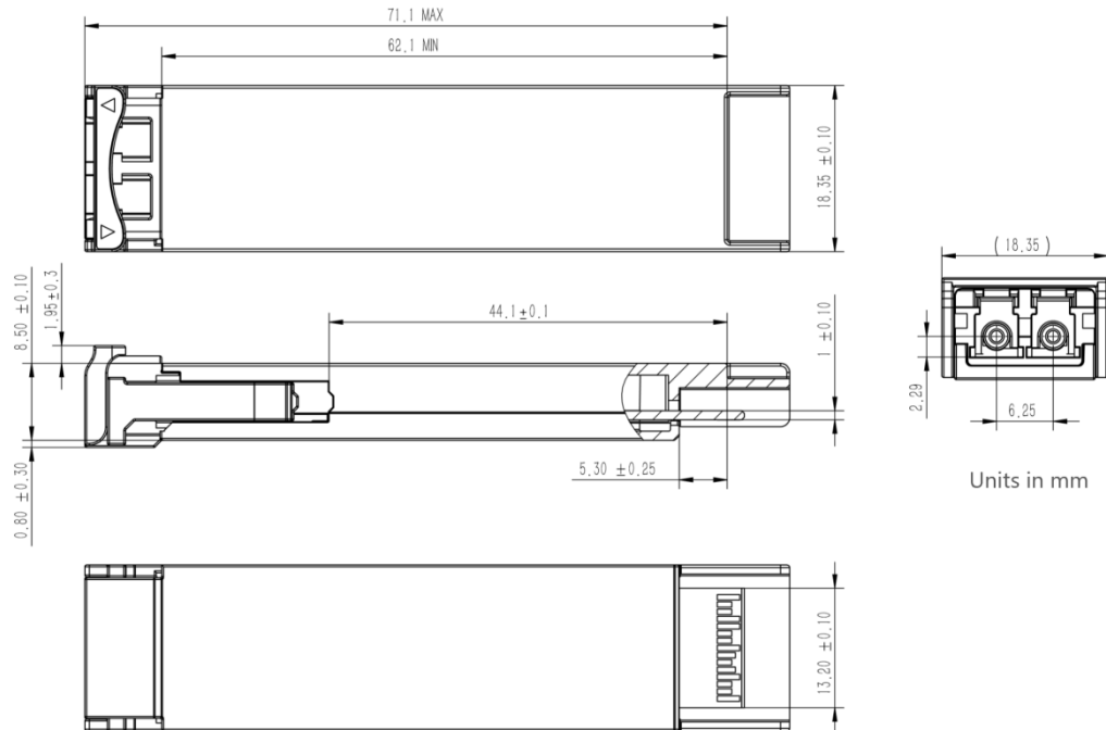
Figure2. Mechanical Outline
