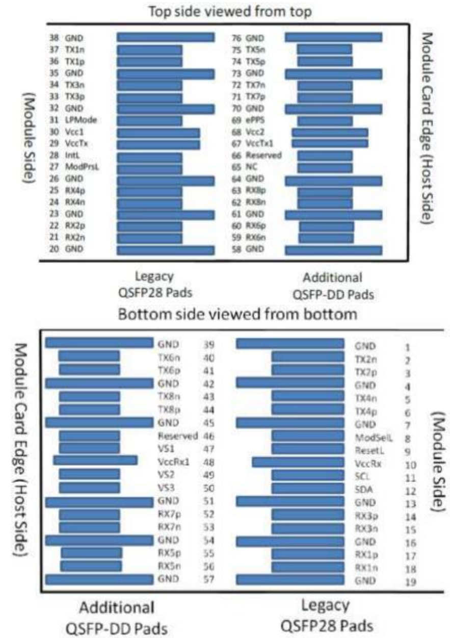
Figure 6: Module pad layout
