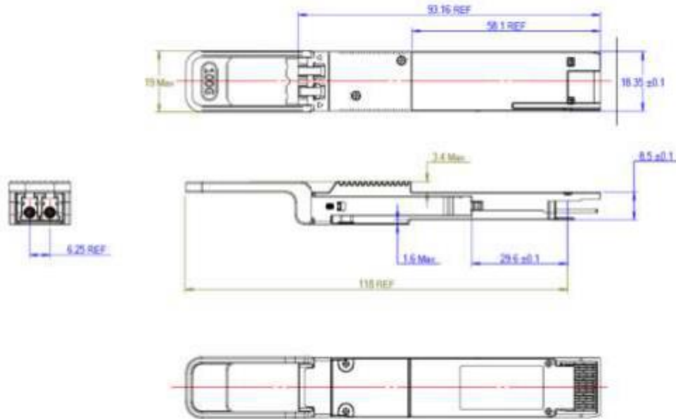
Figure 5: QSFP-DD Module Mechanical drawing
