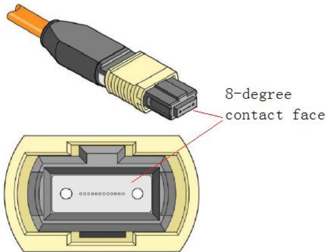
Figure 6. Female MPO Connector with 8-degree End-face
