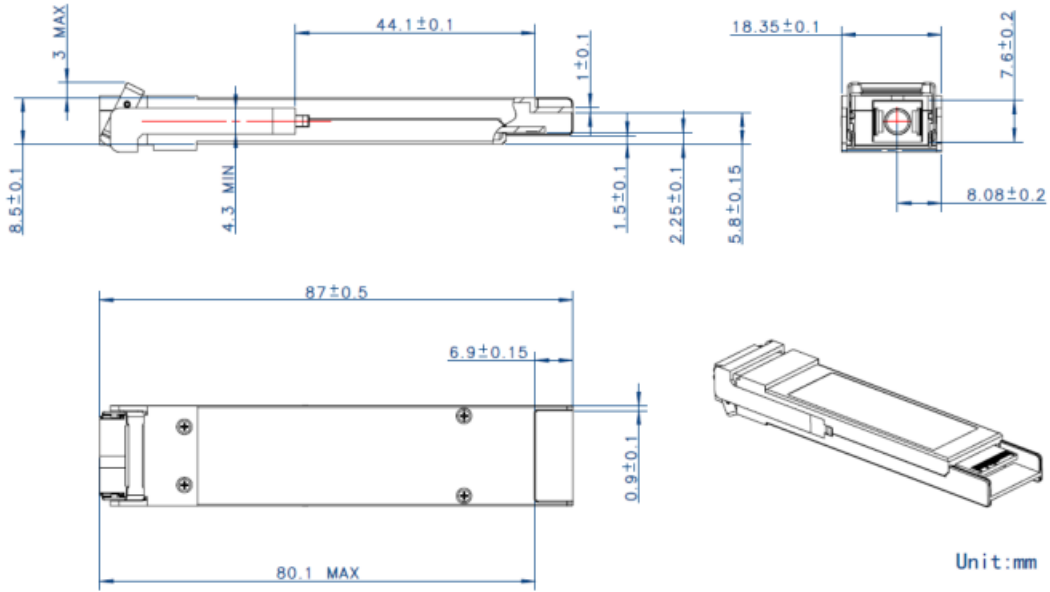
Figure 8: Package Outline
