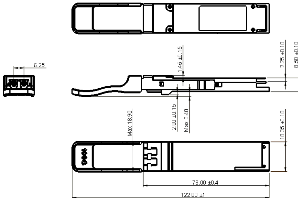
Figure 5. Mechanical Outline
