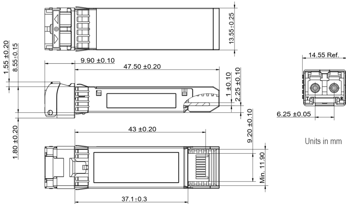
Figure2. Mechanical Outline
