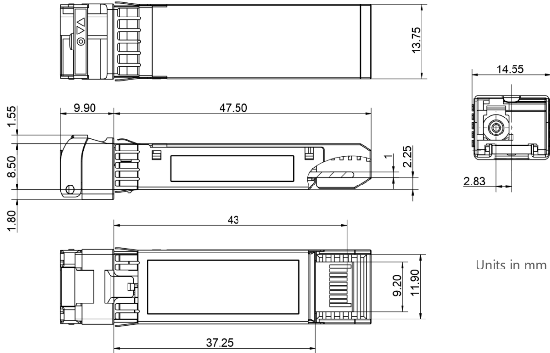
Figure2. Mechanical Outline
