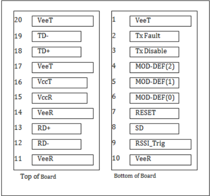
Figure 5: Pin Out Drawing
