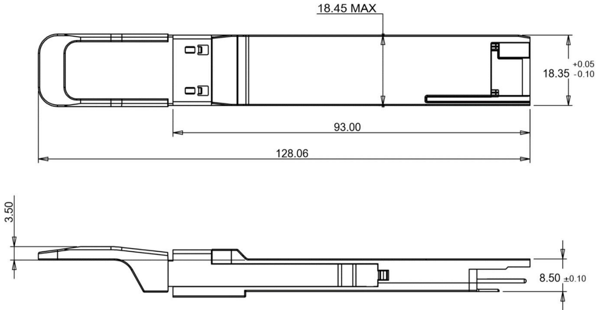
Figure 4. Mechanical Outline
