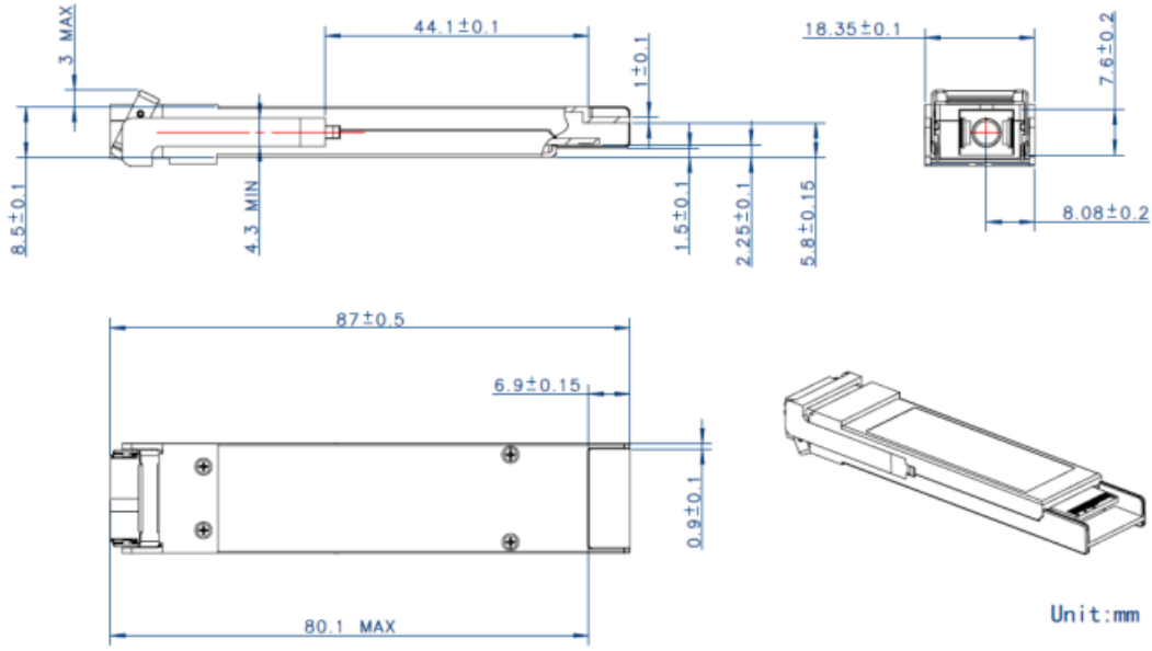
Figure 8: Package Outline
