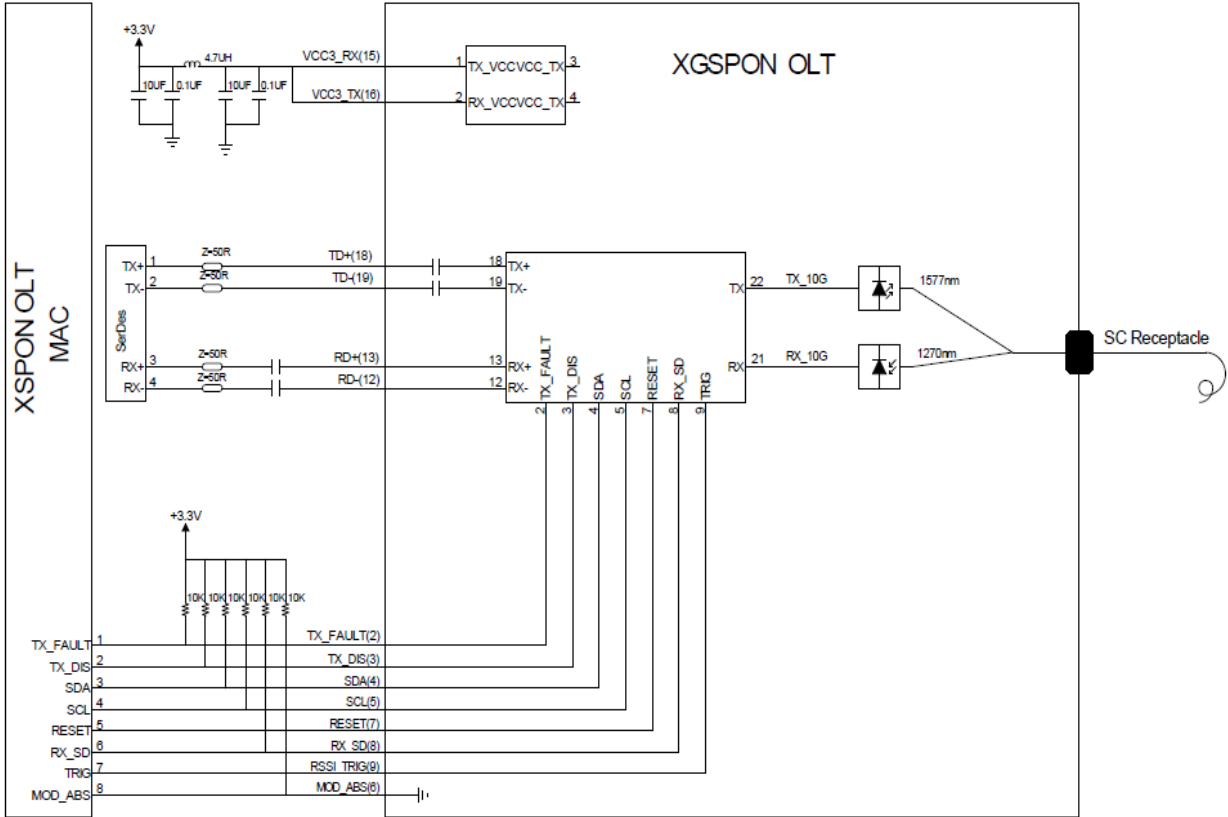
Figure 2. Electrical Interface
