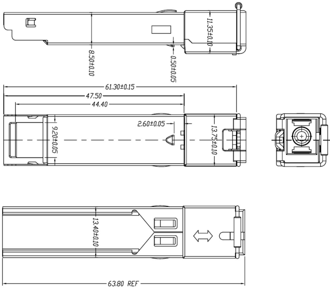
Figure 6 Package Outline
