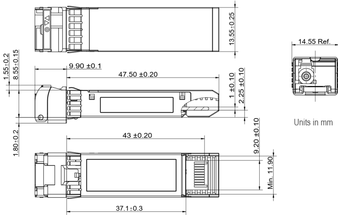
Figure2. Mechanical Outline
